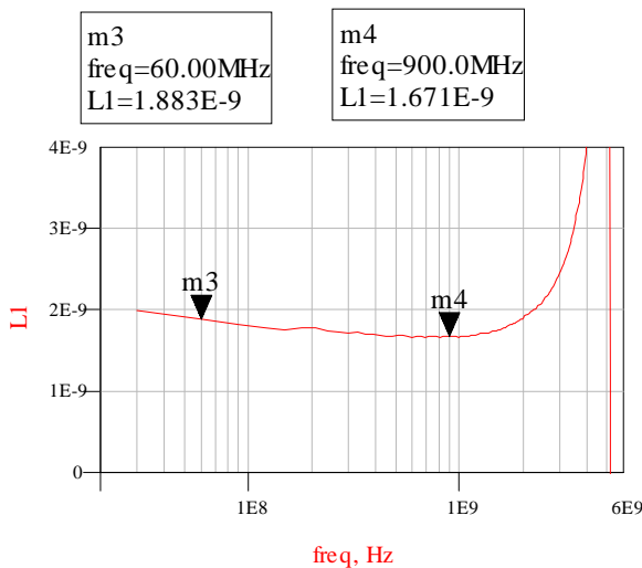
- Inductance for Leeno pin-
